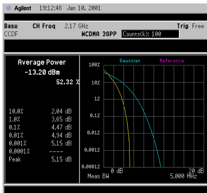
Figure 2-5 Power Stat CCDF Measurement Results
