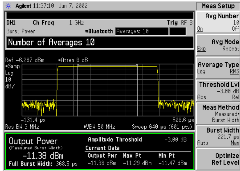
Figure 2-6 Burst Power Measurement Results
