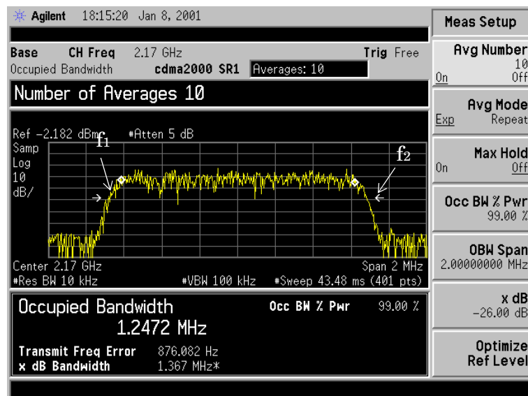
Figure 2-4 Occupied Bandwidth Measurement Results
