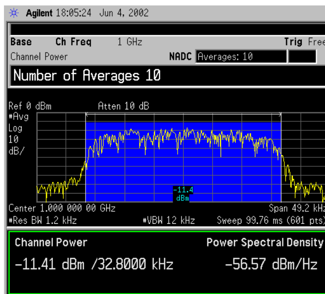
Figure 2-3 PSA Channel Power Measurement Results
