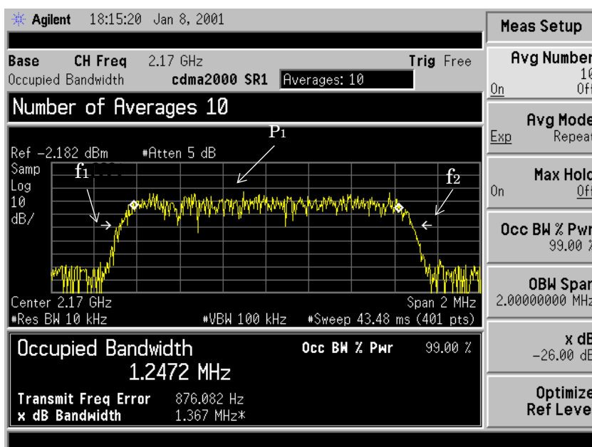
Figure 2-7 Occupied Bandwidth Measurement Results
